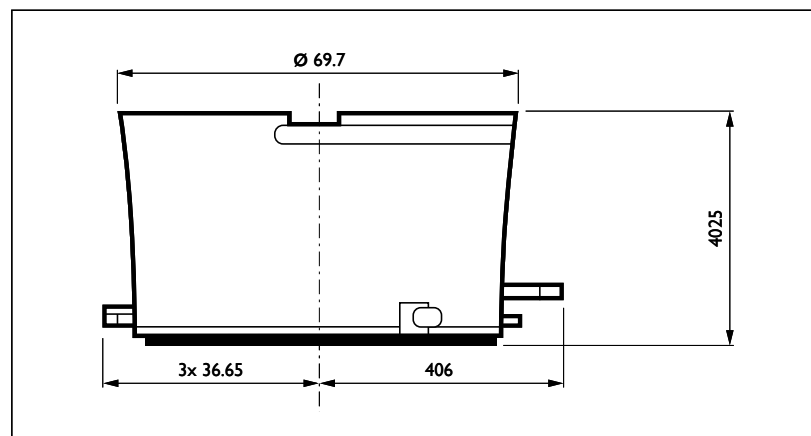
Dimensions Side view Module
