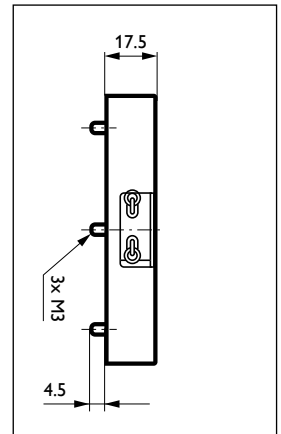
Dimensions Socket profile view
